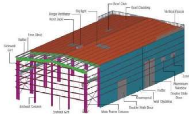
Fig. 1: Components of Pre-Engineered Building
